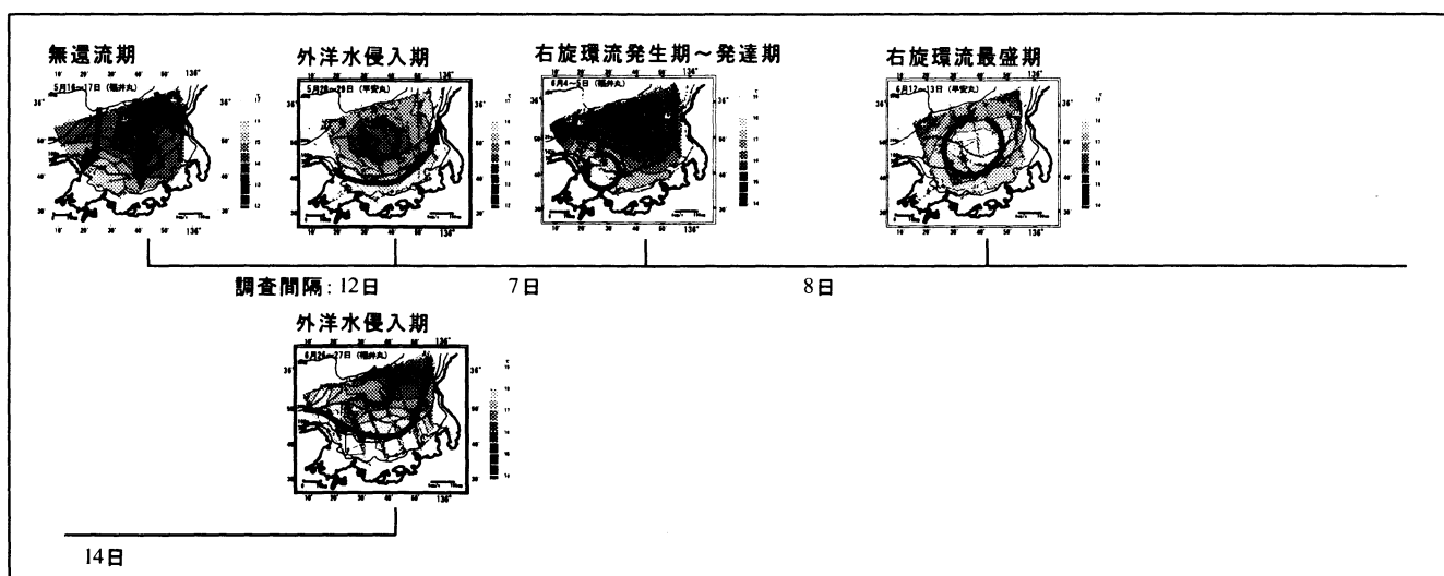
Fig.5 The change of oceanographic conditions between May 16 and June 27.
